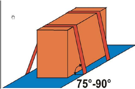
Figure 1A –Top-Over Lashing
