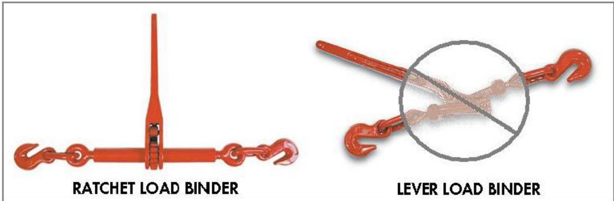
Figure 2 – Ratchet Binders (Approved Standard) Lever Binder ( Prohibited )
